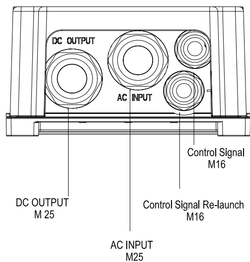
Wire Ports
